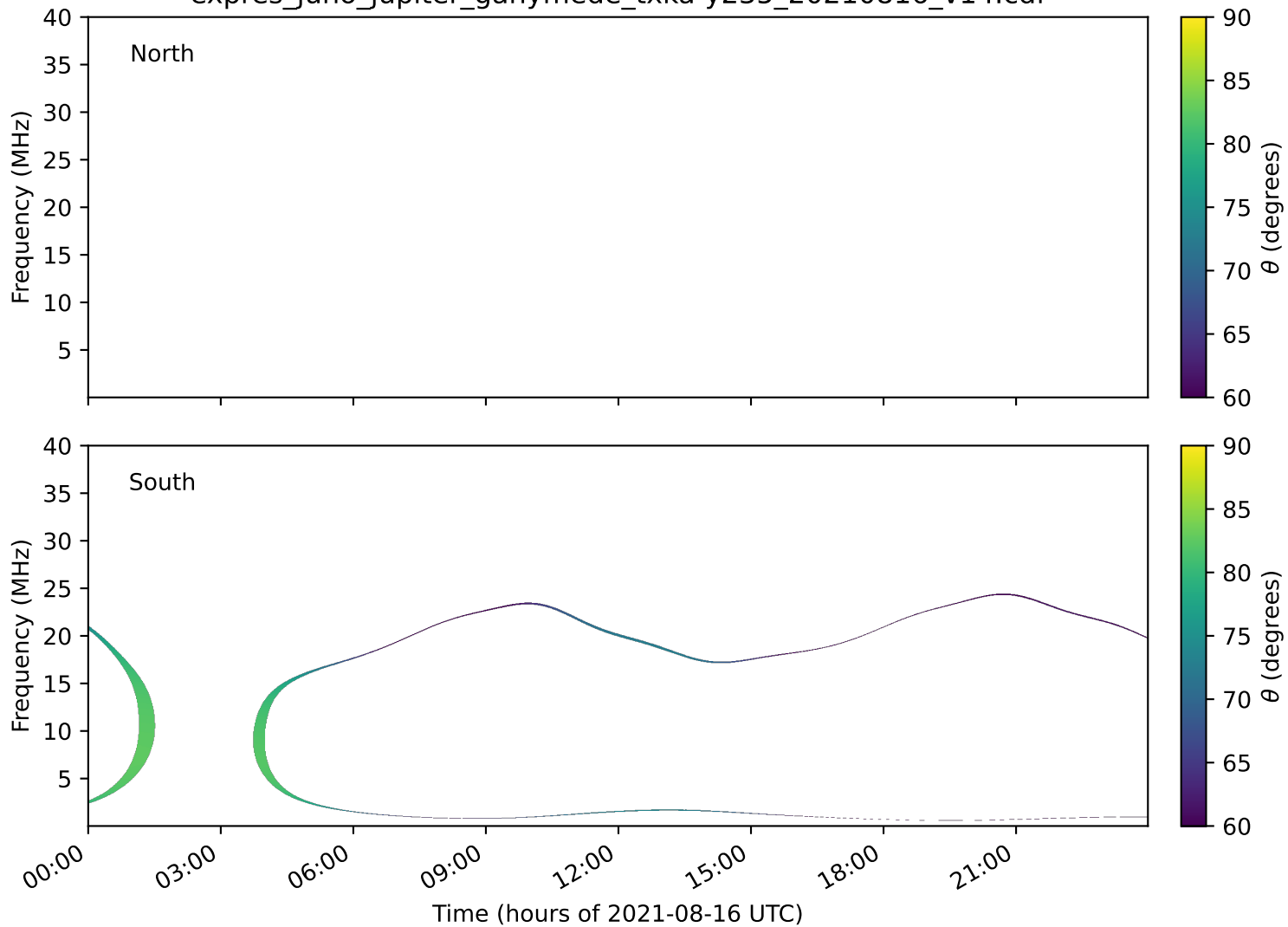
expres_juno_jupiter_ganymede_txka-y235_20210816_v14.cdf
