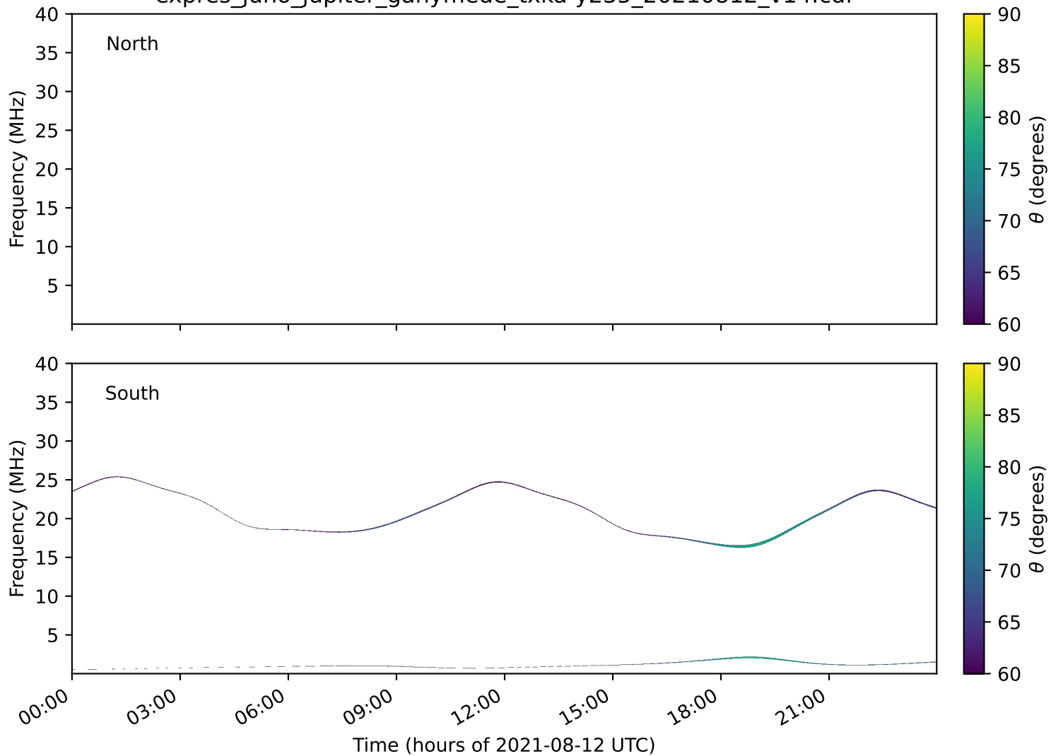
expres_juno_jupiter_ganymede_txka-y235_20210812_v14.cdf
