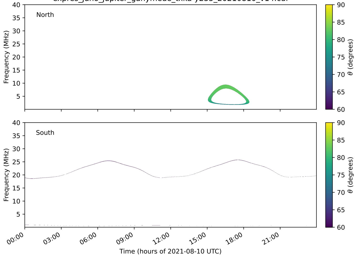
expres_juno_jupiter_ganymede_txka-y235_20210810_v14.cdf
