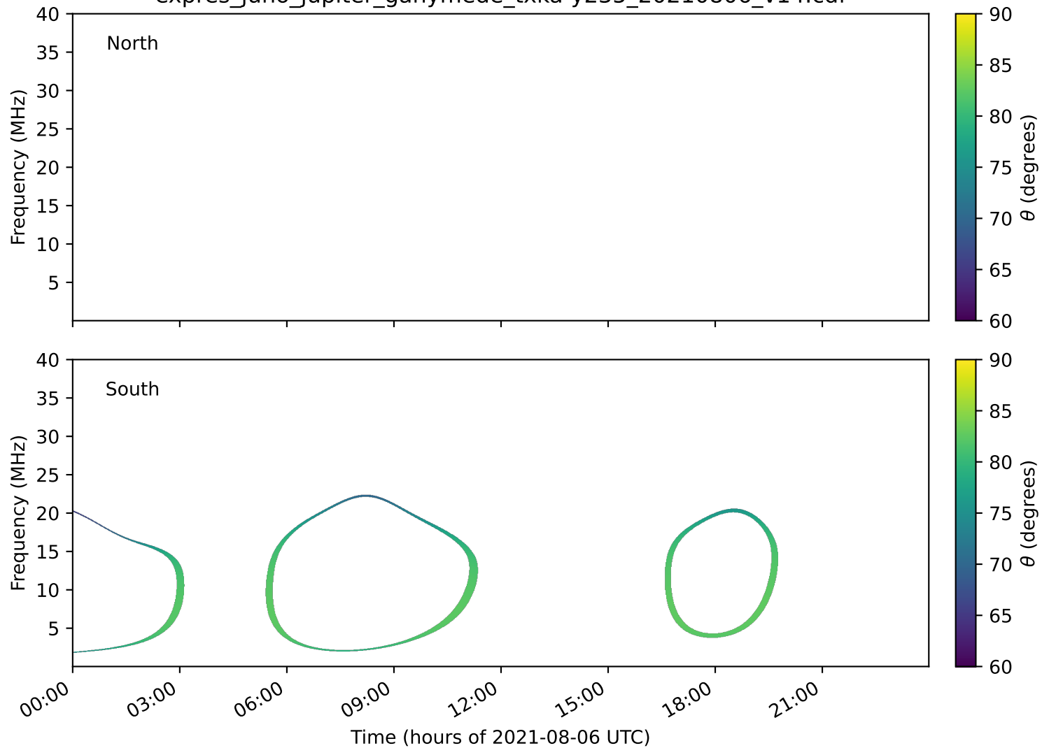
expres_juno_jupiter_ganymede_txka-y235_20210806_v14.cdf
