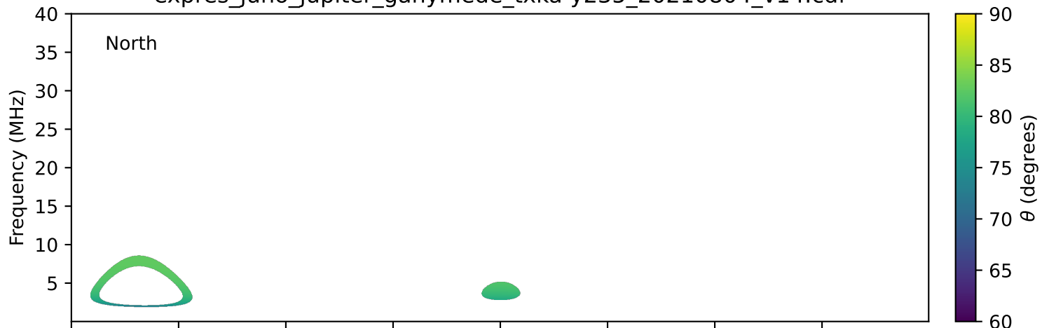
expres_juno_jupiter_ganymede_txka-y235_20210804_v14.cdf
