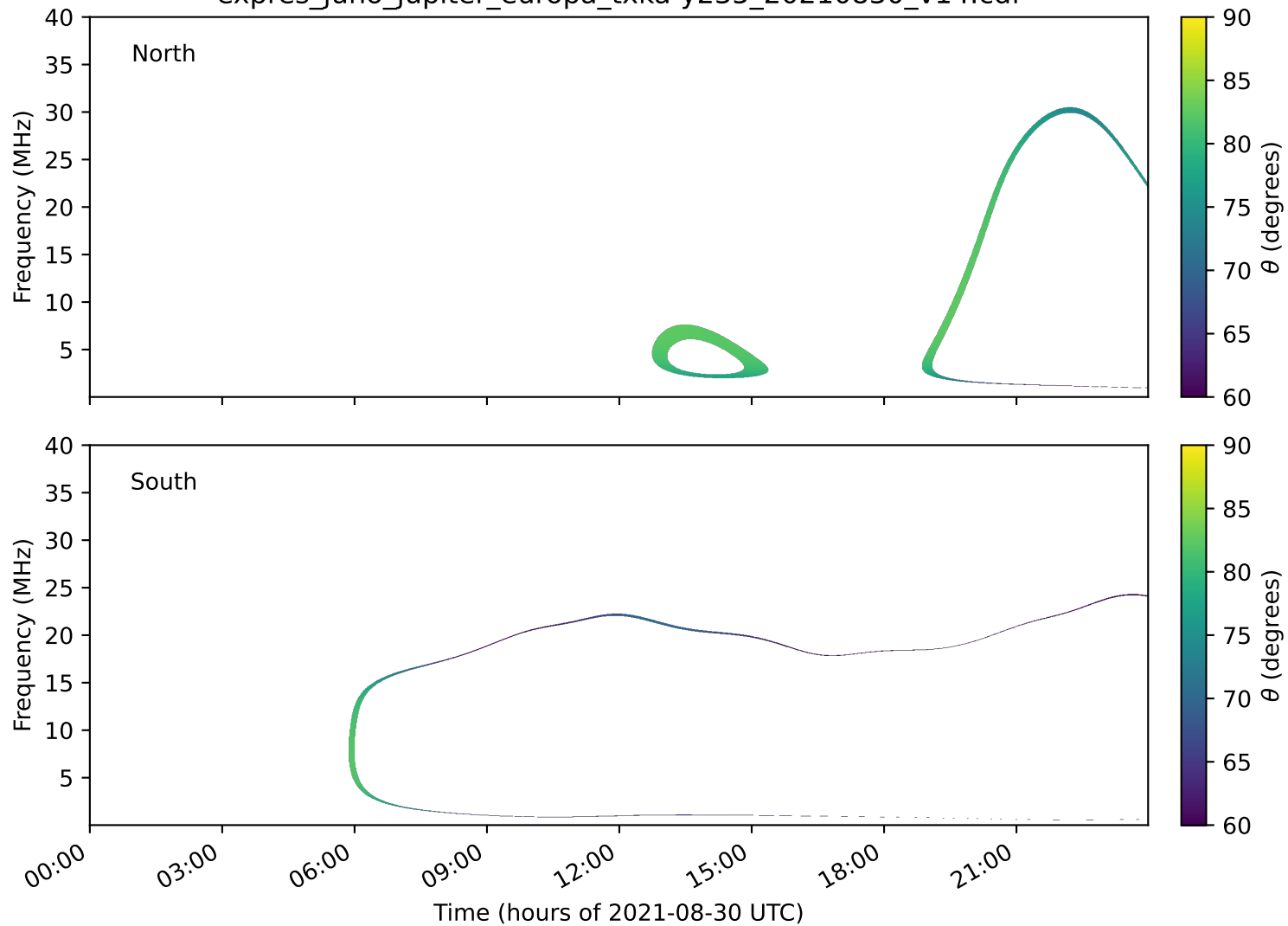
expres_juno_jupiter_europa_txka-y235_20210830_v14.cdf
