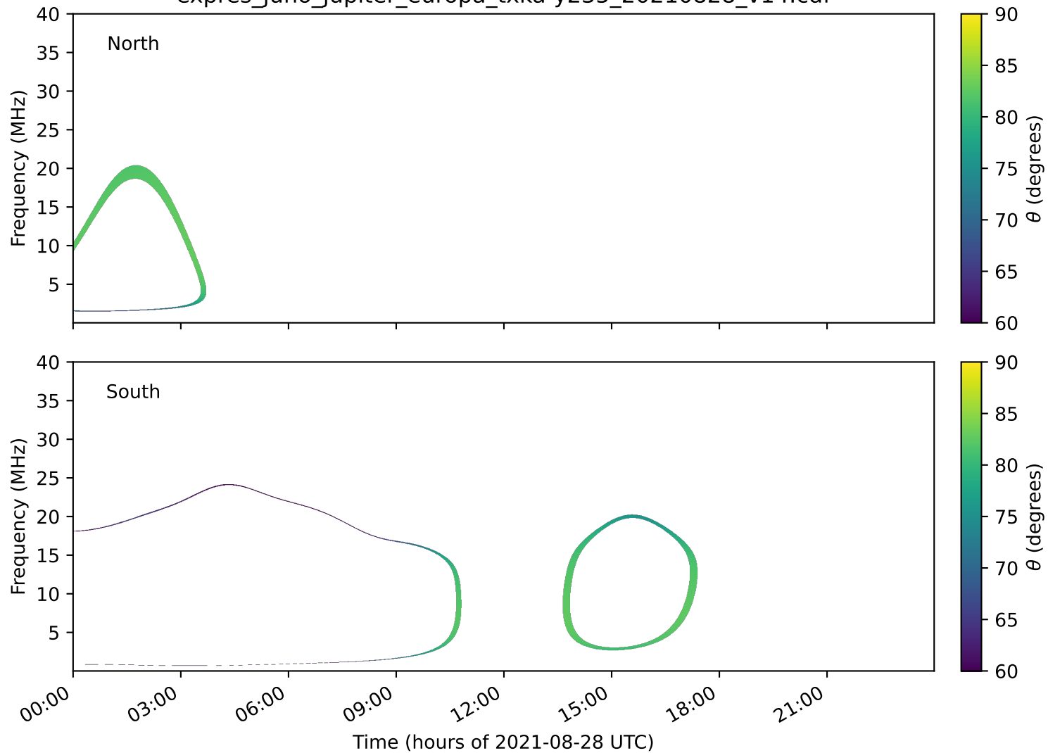
expres_juno_jupiter_europa_txka-y235_20210828_v14.cdf
