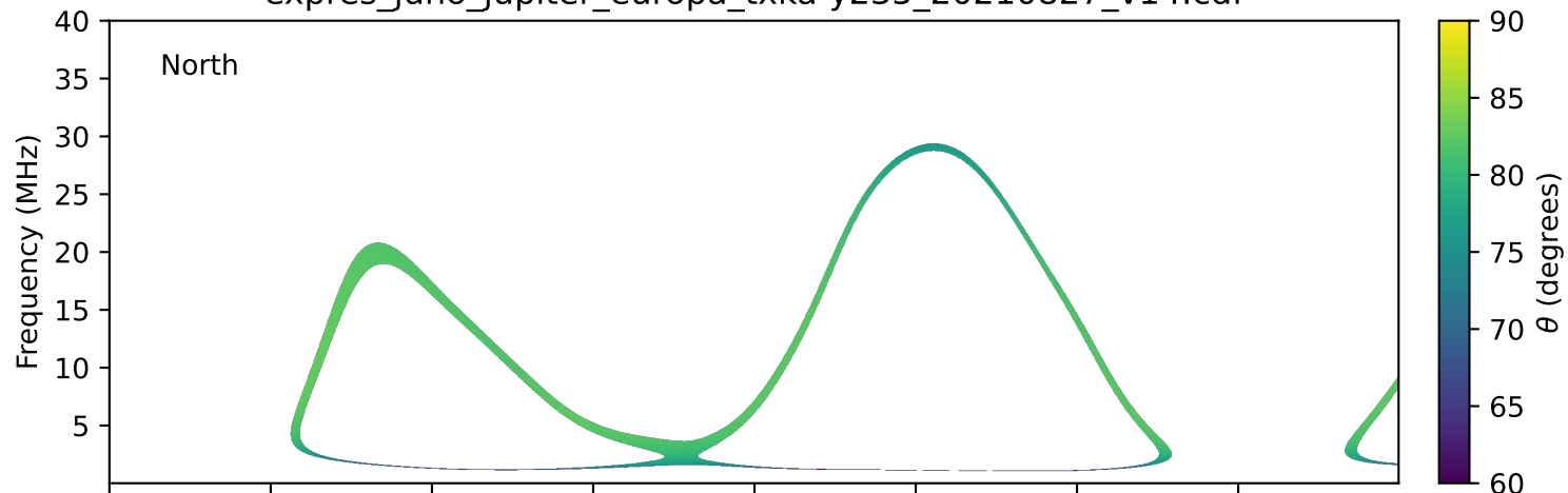
expres_juno_jupiter_europa_txka-y235_20210827_v14.cdf
