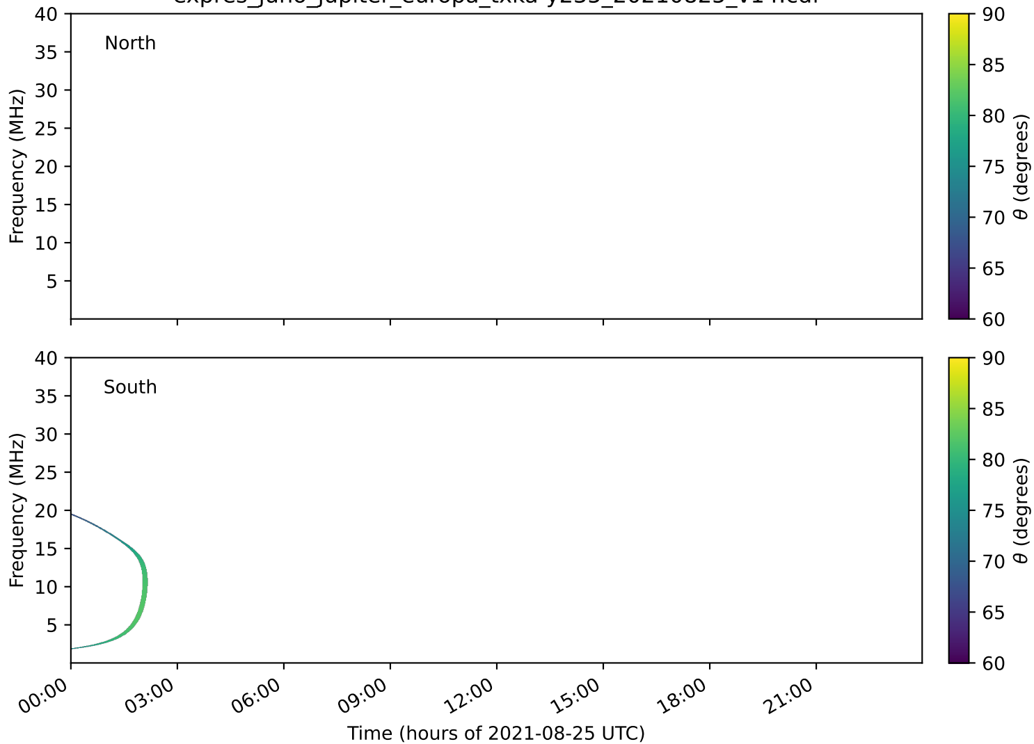
expres_juno_jupiter_europa_txka-y235_20210825_v14.cdf
