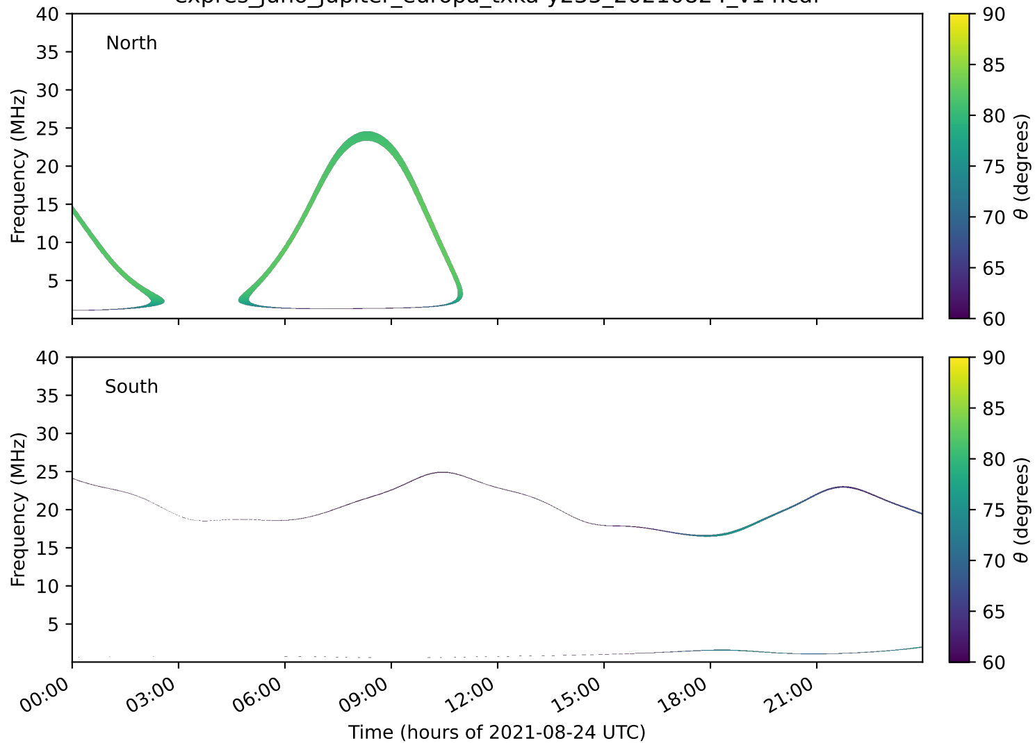
expres_juno_jupiter_europa_txka-y235_20210824_v14.cdf
