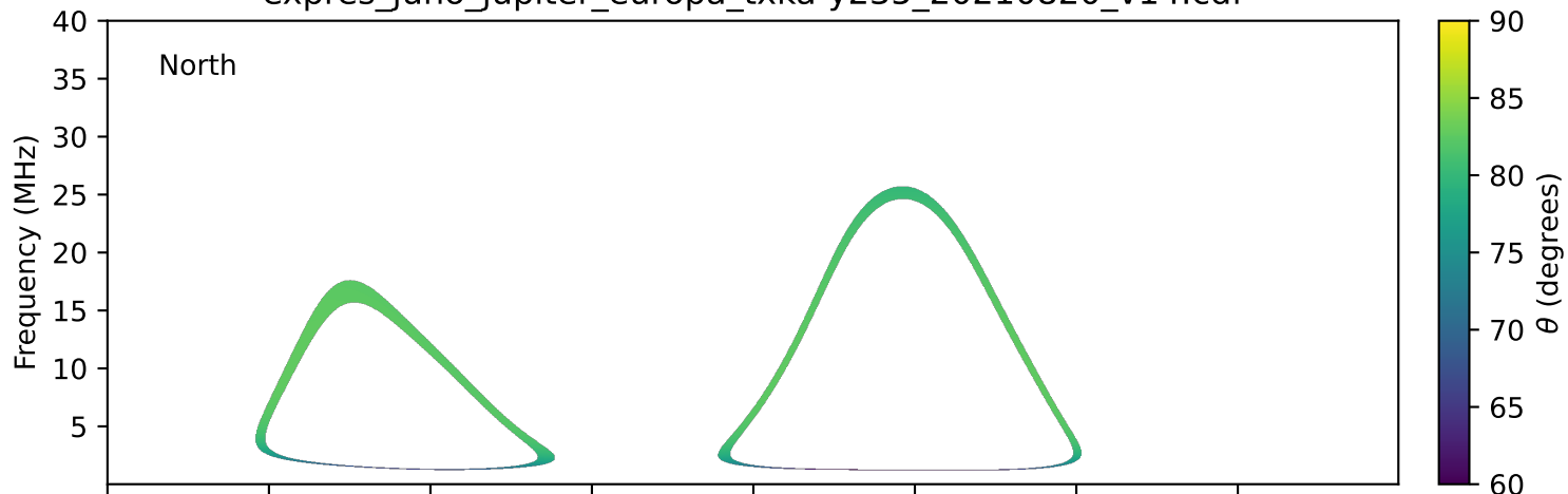
expres_juno_jupiter_europa_txka-y235_20210820_v14.cdf
