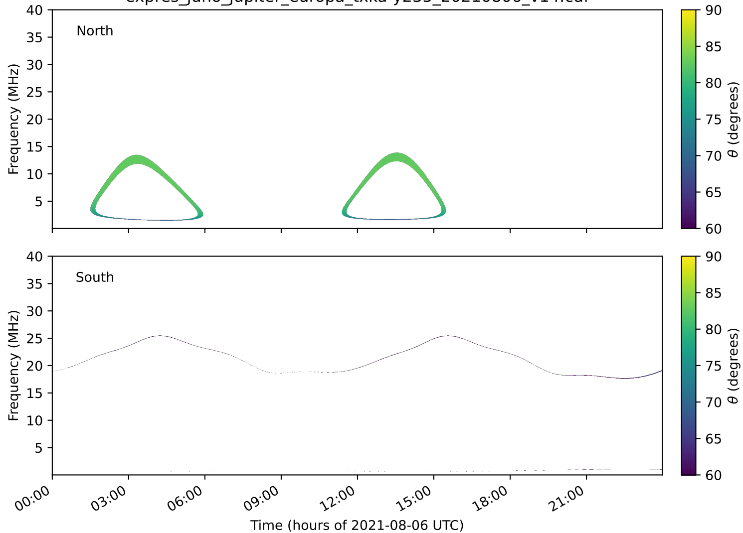
expres_juno_jupiter_europa_txka-y235_20210806_v14.cdf
