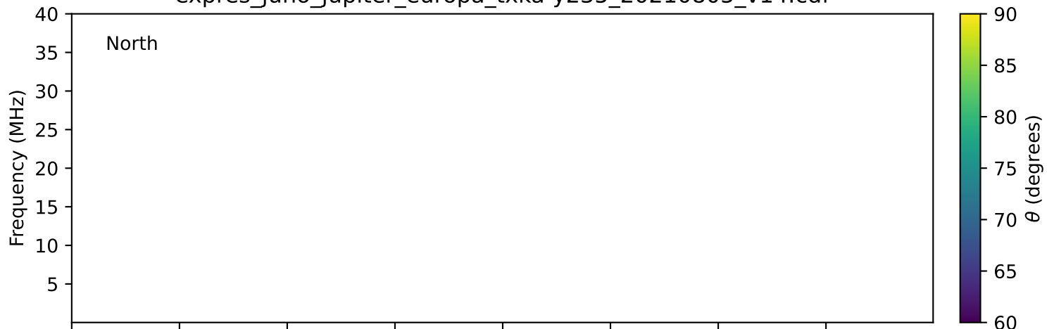
expres_juno_jupiter_europa_txka-y235_20210805_v14.cdf
