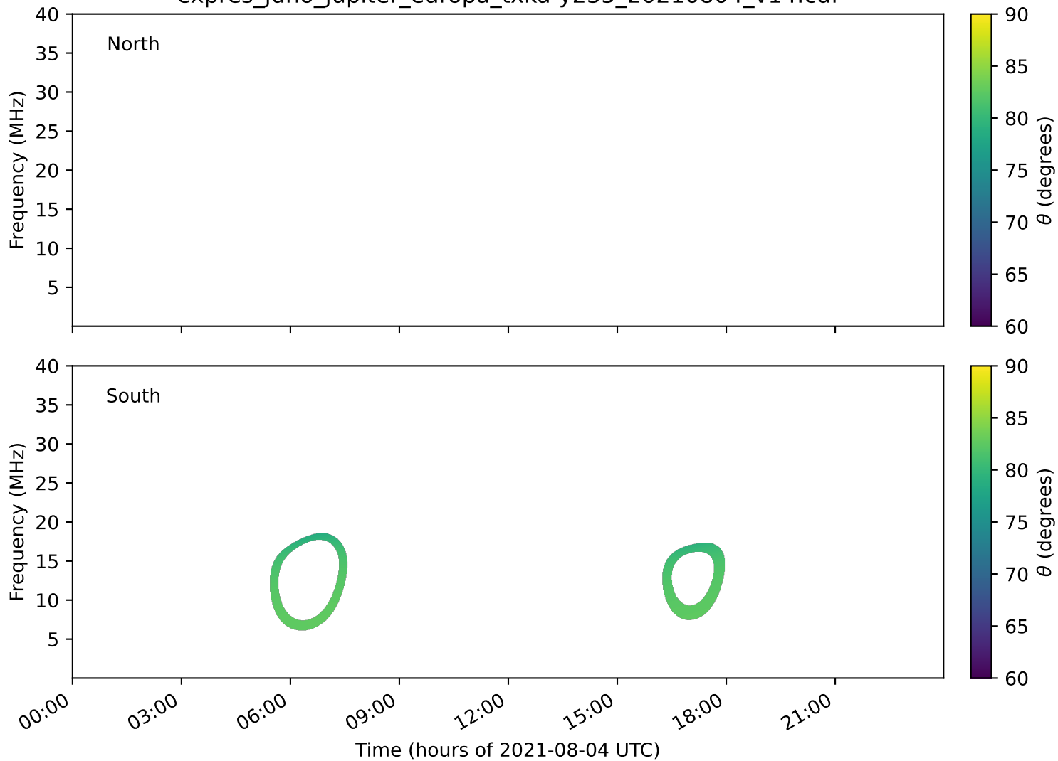
expres_juno_jupiter_europa_txka-y235_20210804_v14.cdf
