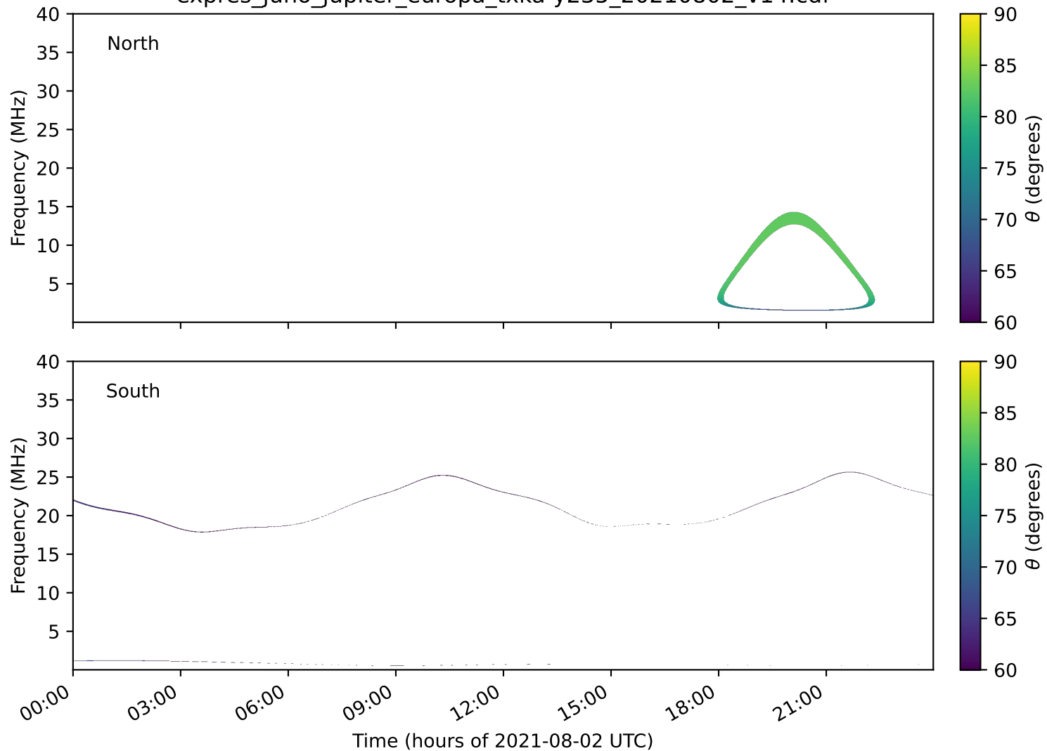
expres_juno_jupiter_europa_txka-y235_20210802_v14.cdf
