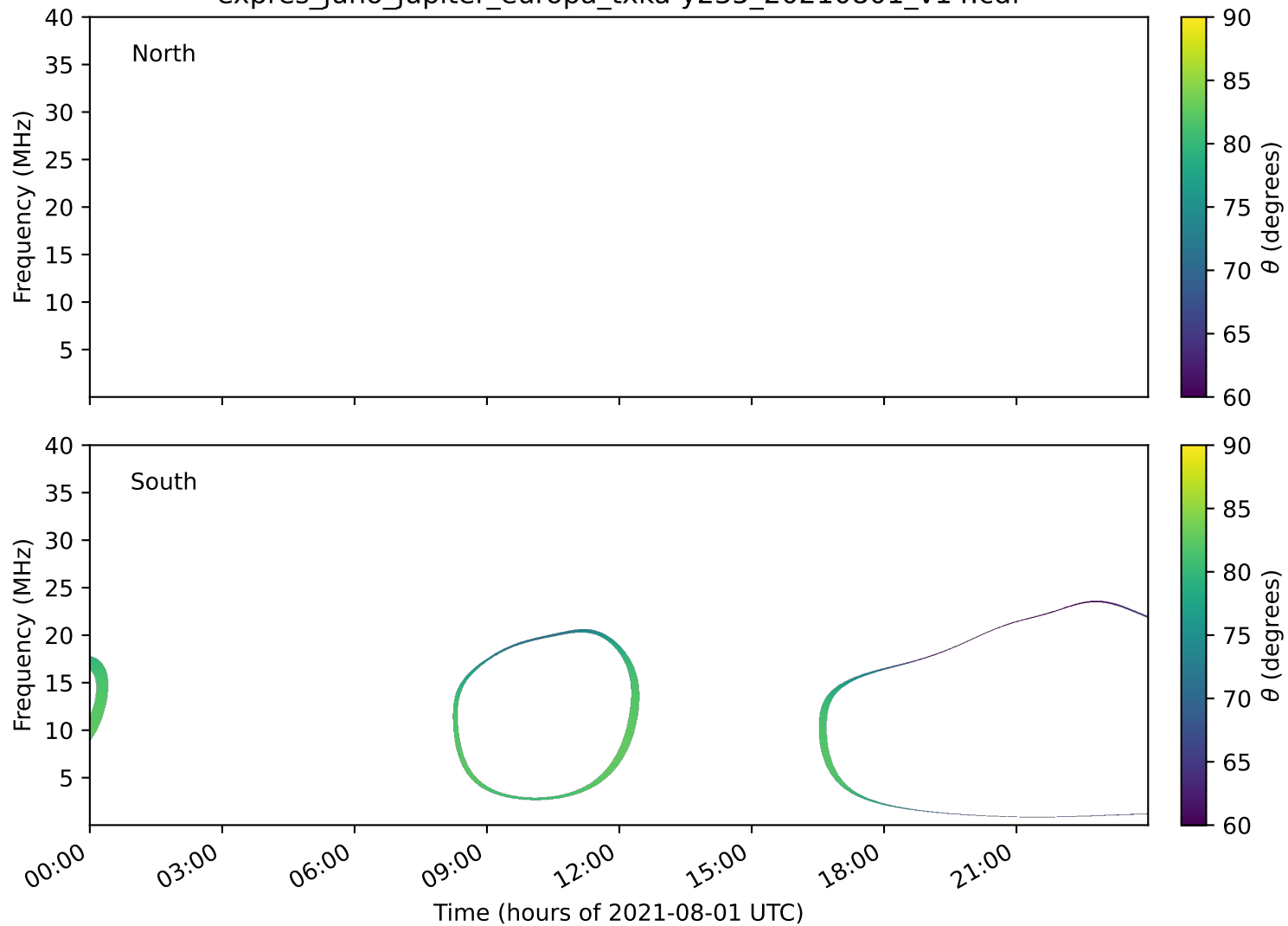
expres_juno_jupiter_europa_txka-y235_20210801_v14.cdf
