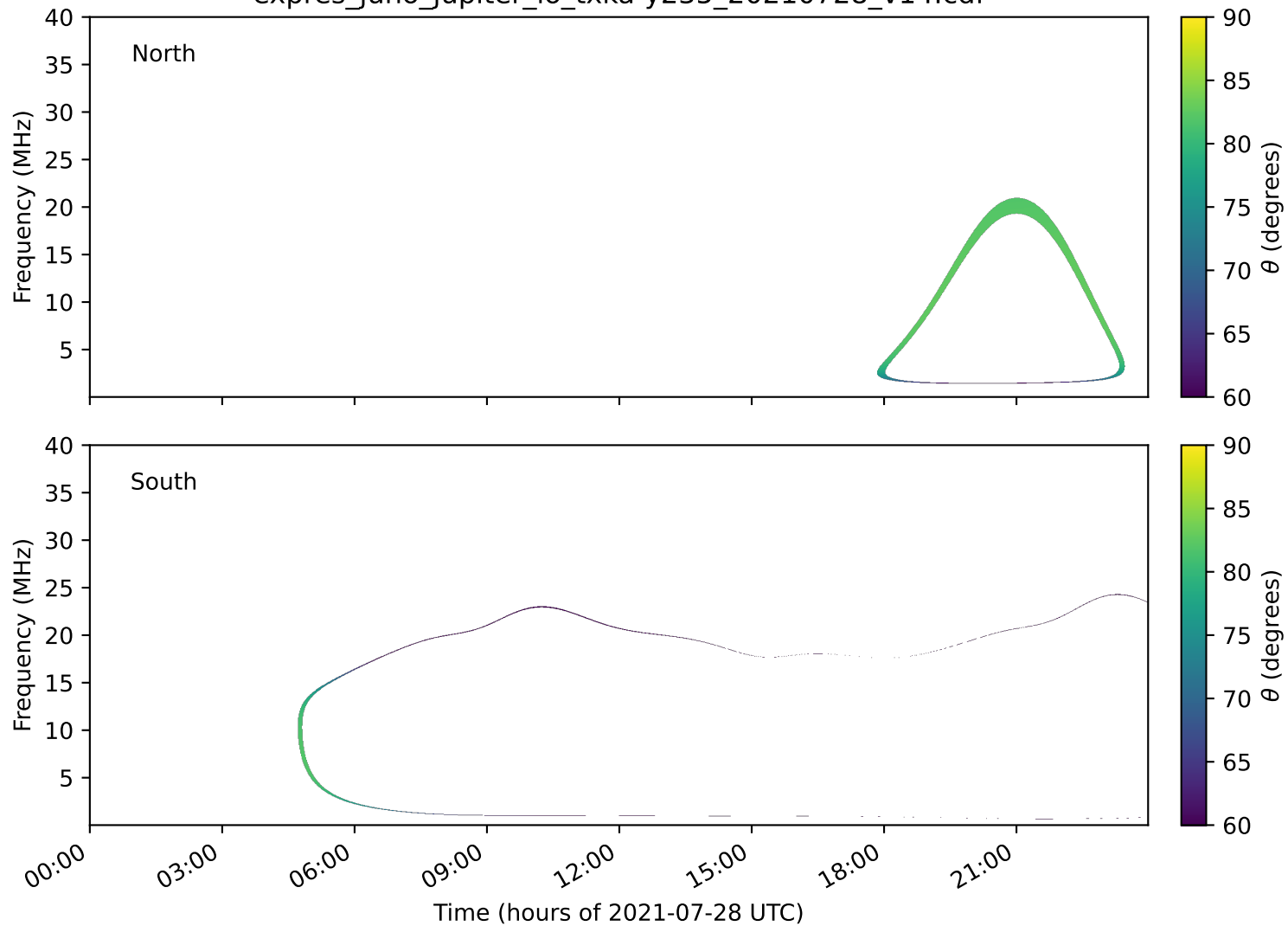
expres_juno_jupiter_io_txka-y235_20210728_v14.cdf
