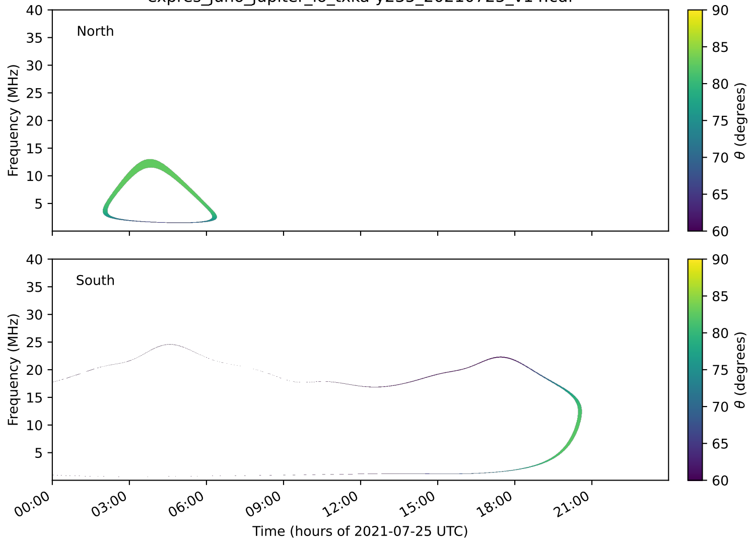
expres_juno_jupiter_io_txka-y235_20210725_v14.cdf
