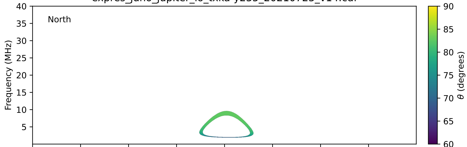
expres_juno_jupiter_io_txka-y235_20210723_v14.cdf
