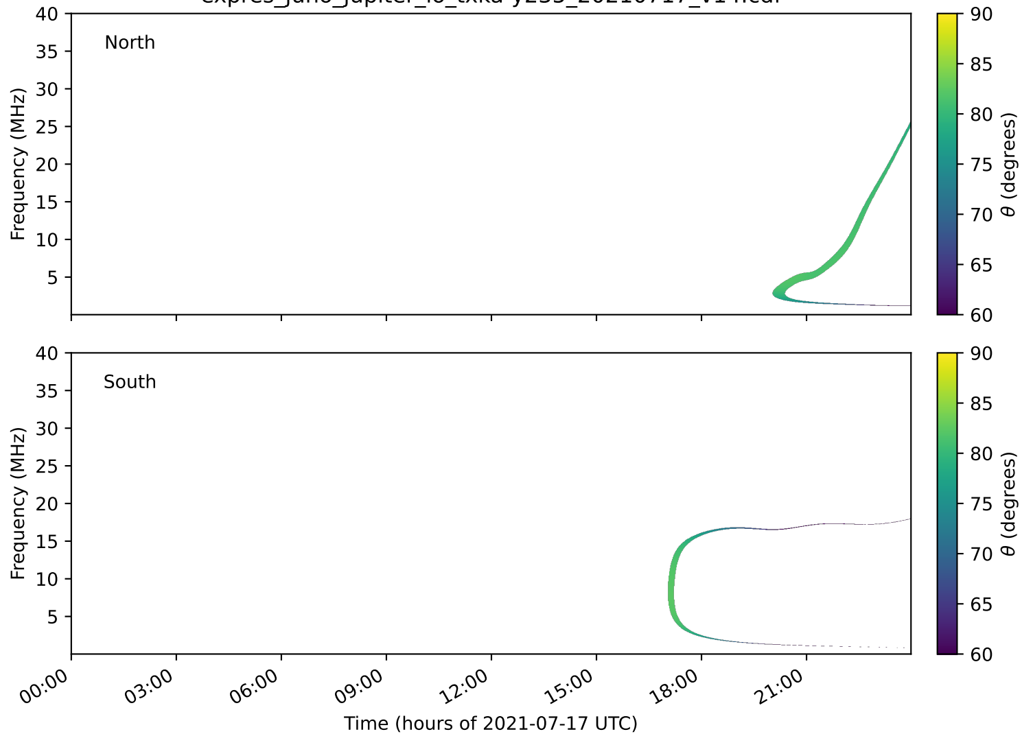
expres_juno_jupiter_io_txka-y235_20210717_v14.cdf
