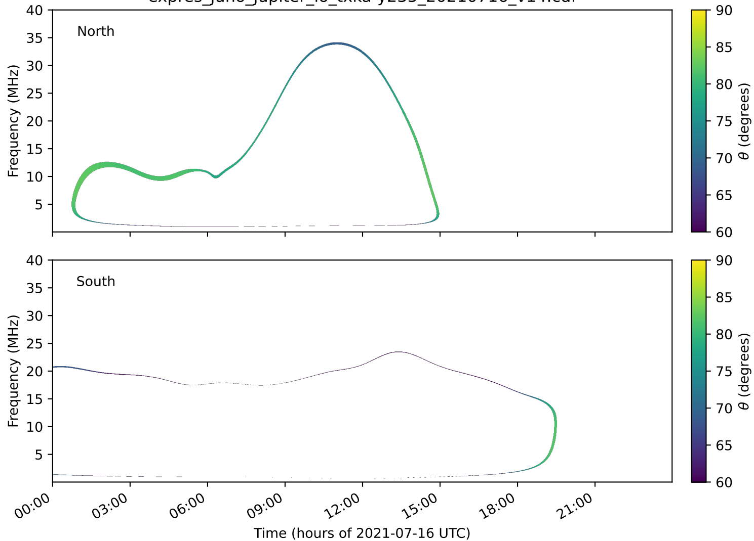
expres_juno_jupiter_io_txka-y235_20210716_v14.cdf
