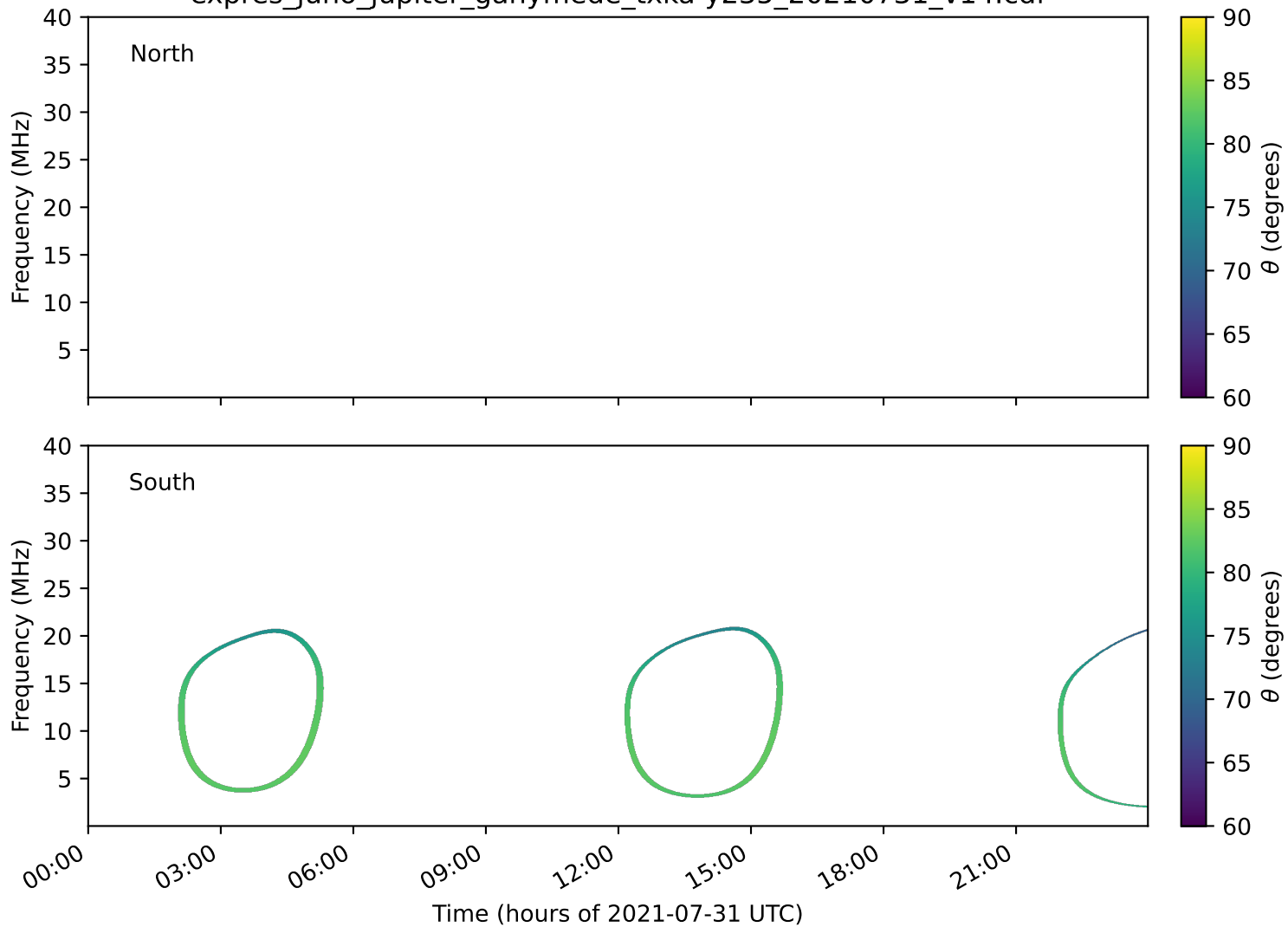
expres_juno_jupiter_ganymede_txka-y235_20210731_v14.cdf
