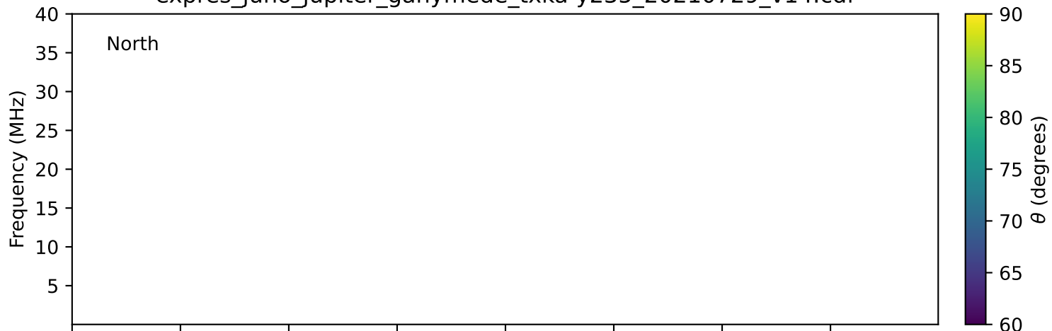
expres_juno_jupiter_ganymede_txka-y235_20210729_v14.cdf
