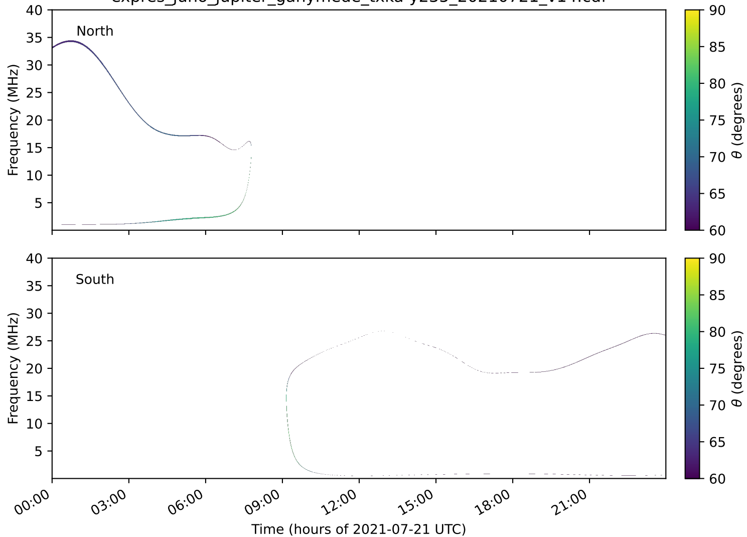
expres_juno_jupiter_ganymede_txka-y235_20210721_v14.cdf
