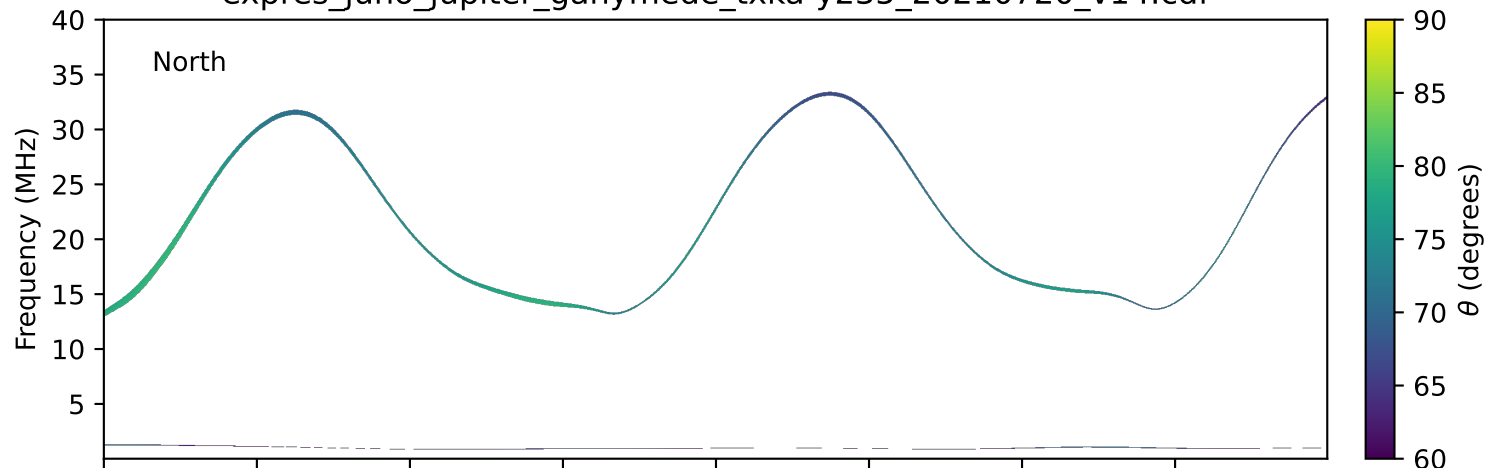
expres_juno_jupiter_ganymede_txka-y235_20210720_v14.cdf
