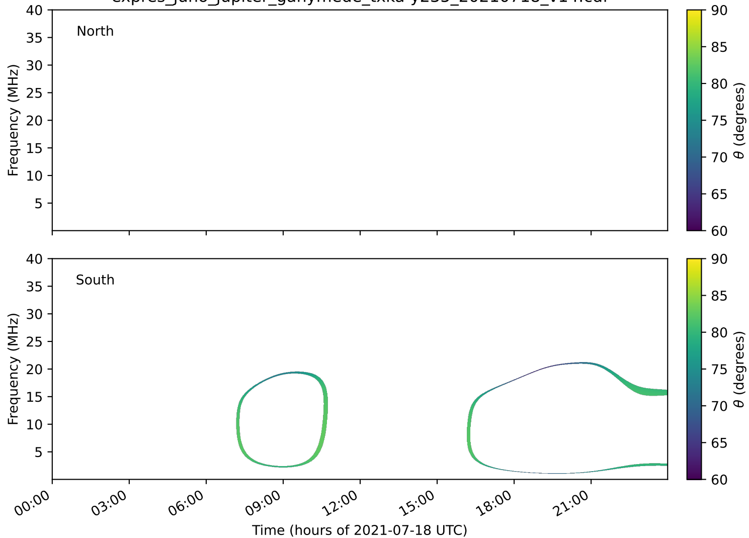
expres_juno_jupiter_ganymede_txka-y235_20210718_v14.cdf
