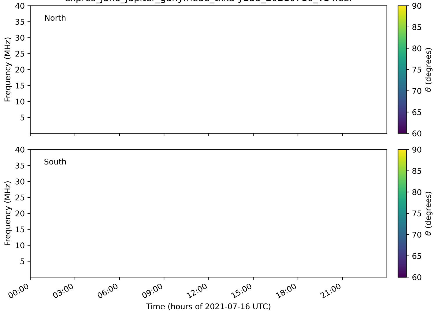
expres_juno_jupiter_ganymede_txka-y235_20210716_v14.cdf
