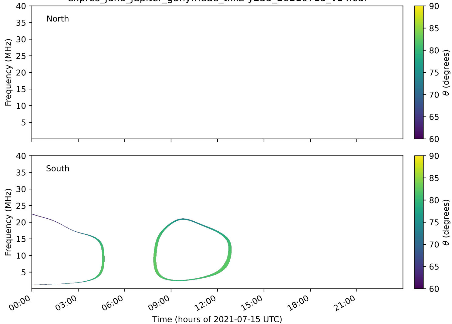
expres_juno_jupiter_ganymede_txka-y235_20210715_v14.cdf
