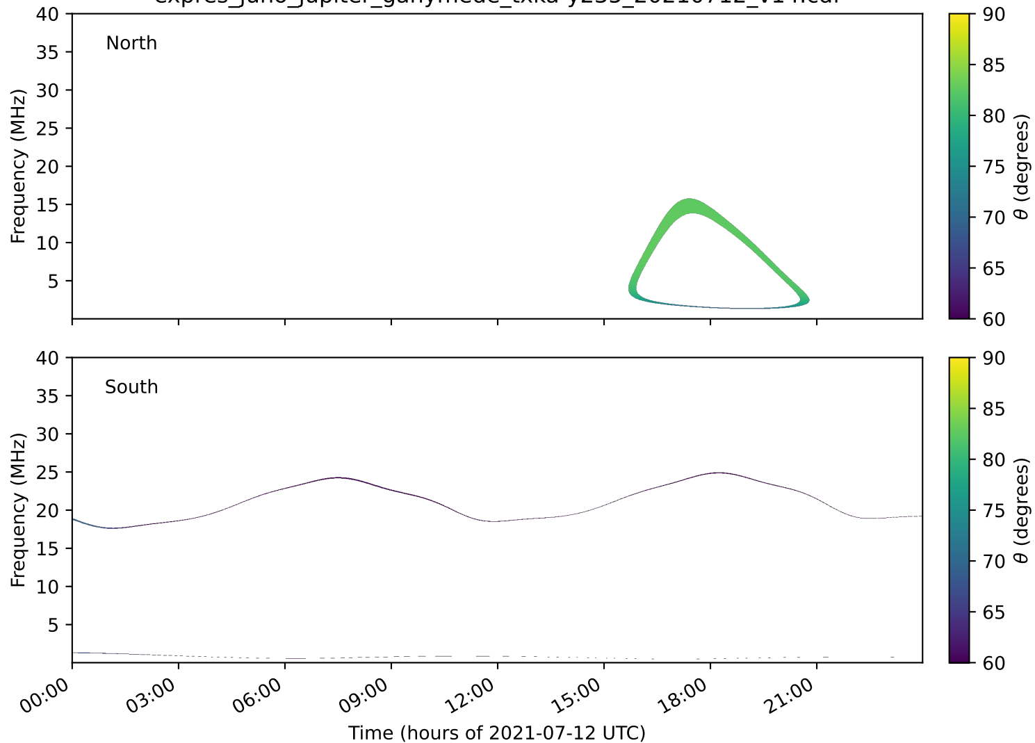
expres_juno_jupiter_ganymede_txka-y235_20210712_v14.cdf
