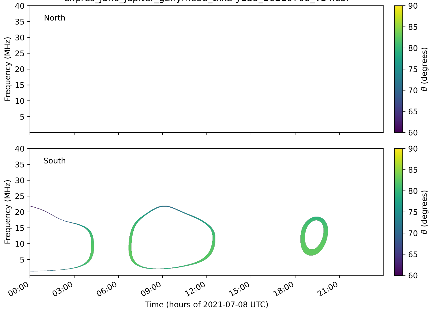
expres_juno_jupiter_ganymede_txka-y235_20210708_v14.cdf
