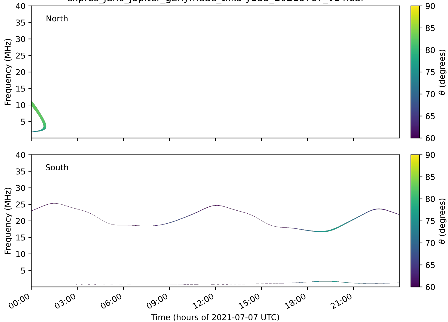
expres_juno_jupiter_ganymede_txka-y235_20210707_v14.cdf
