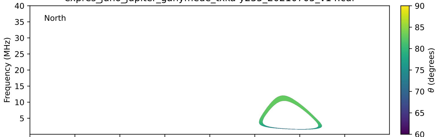
expres_juno_jupiter_ganymede_txka-y235_20210705_v14.cdf
