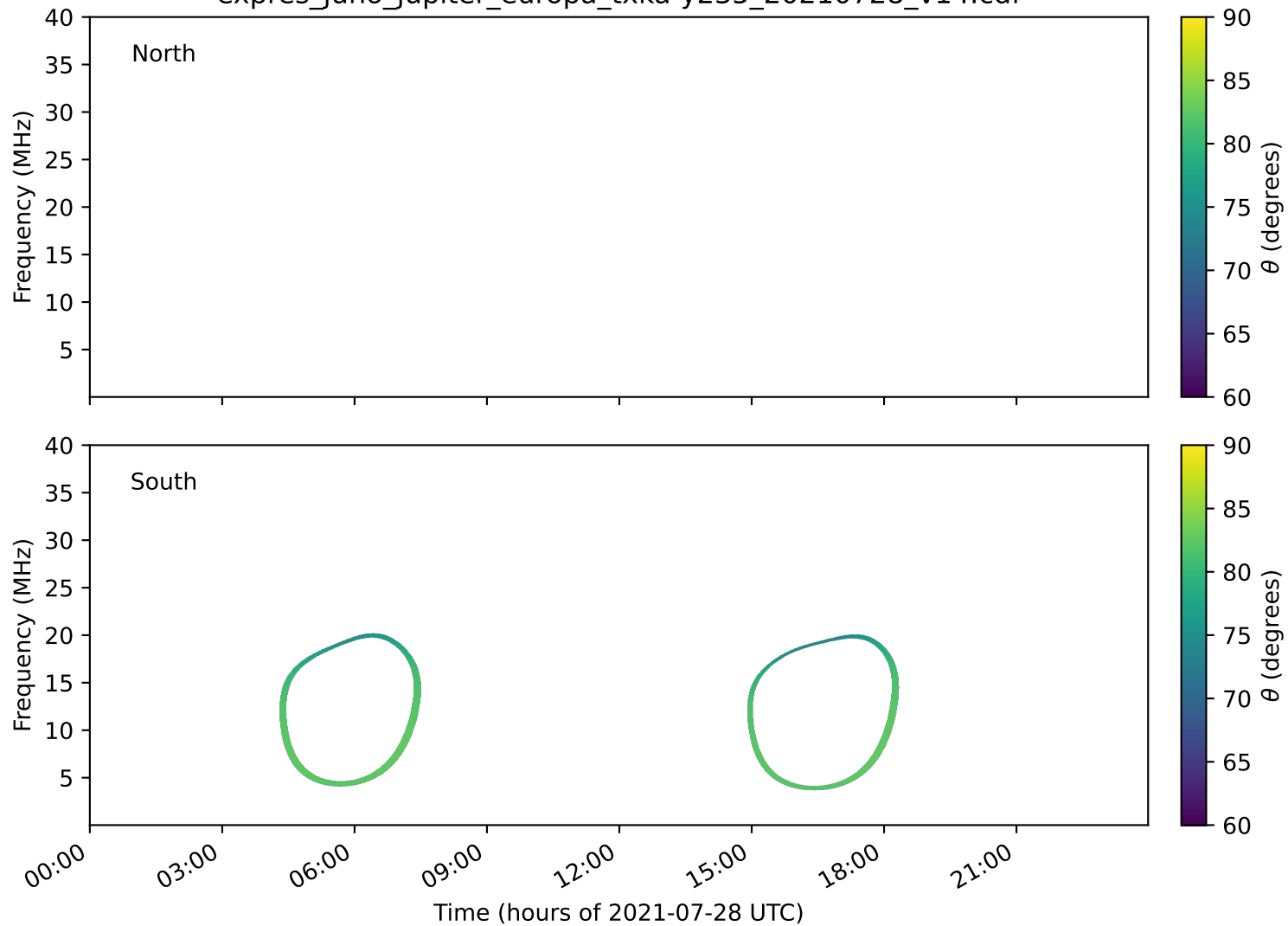
expres_juno_jupiter_europa_txka-y235_20210728_v14.cdf
