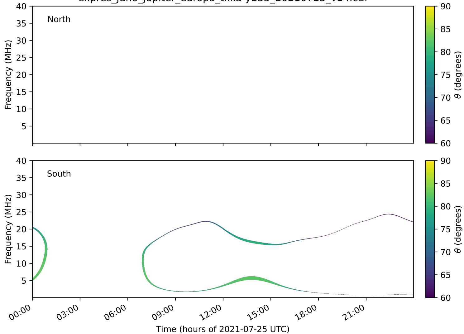
expres_juno_jupiter_europa_txka-y235_20210725_v14.cdf
