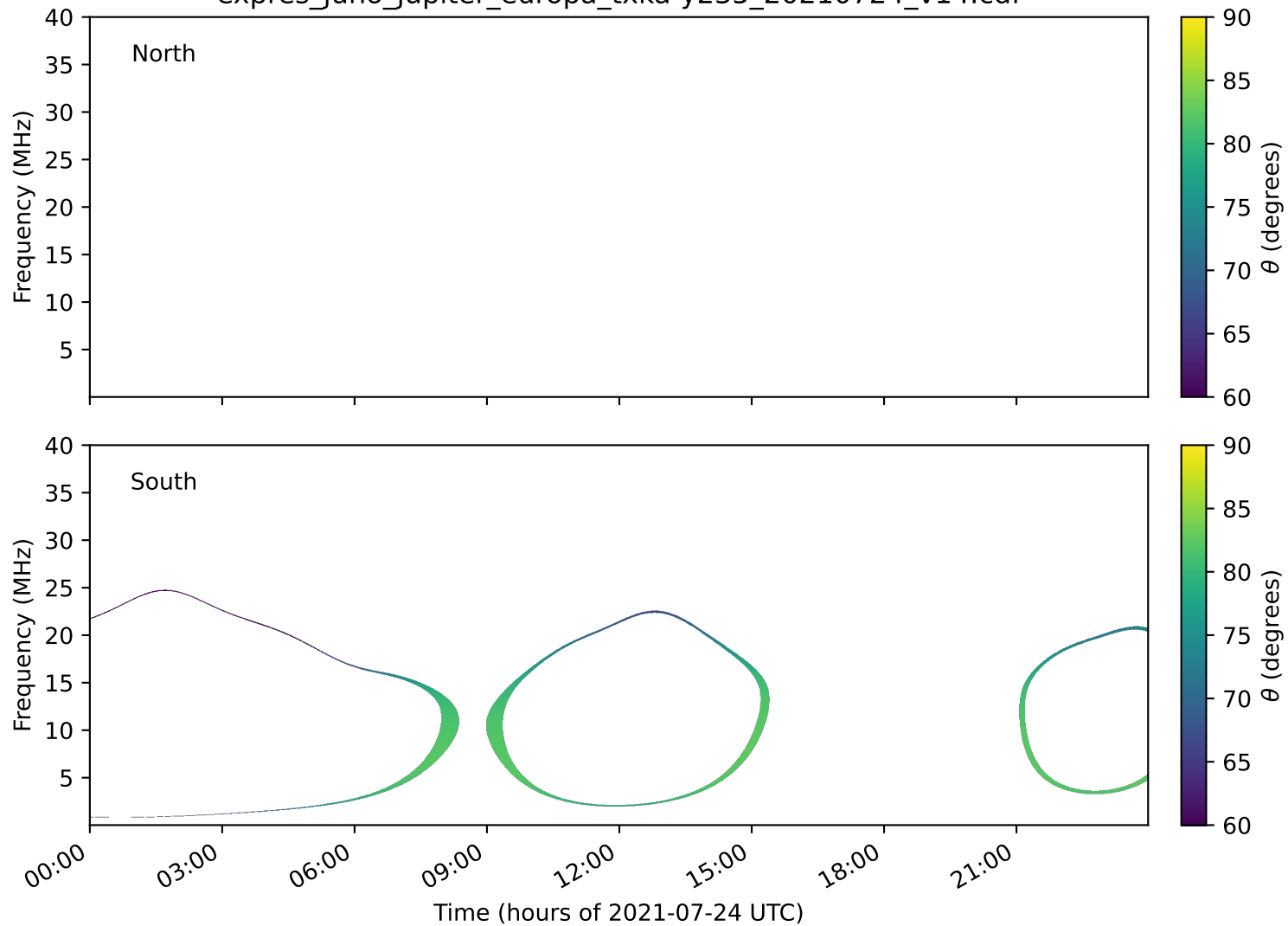
expres_juno_jupiter_europa_txka-y235_20210724_v14.cdf
