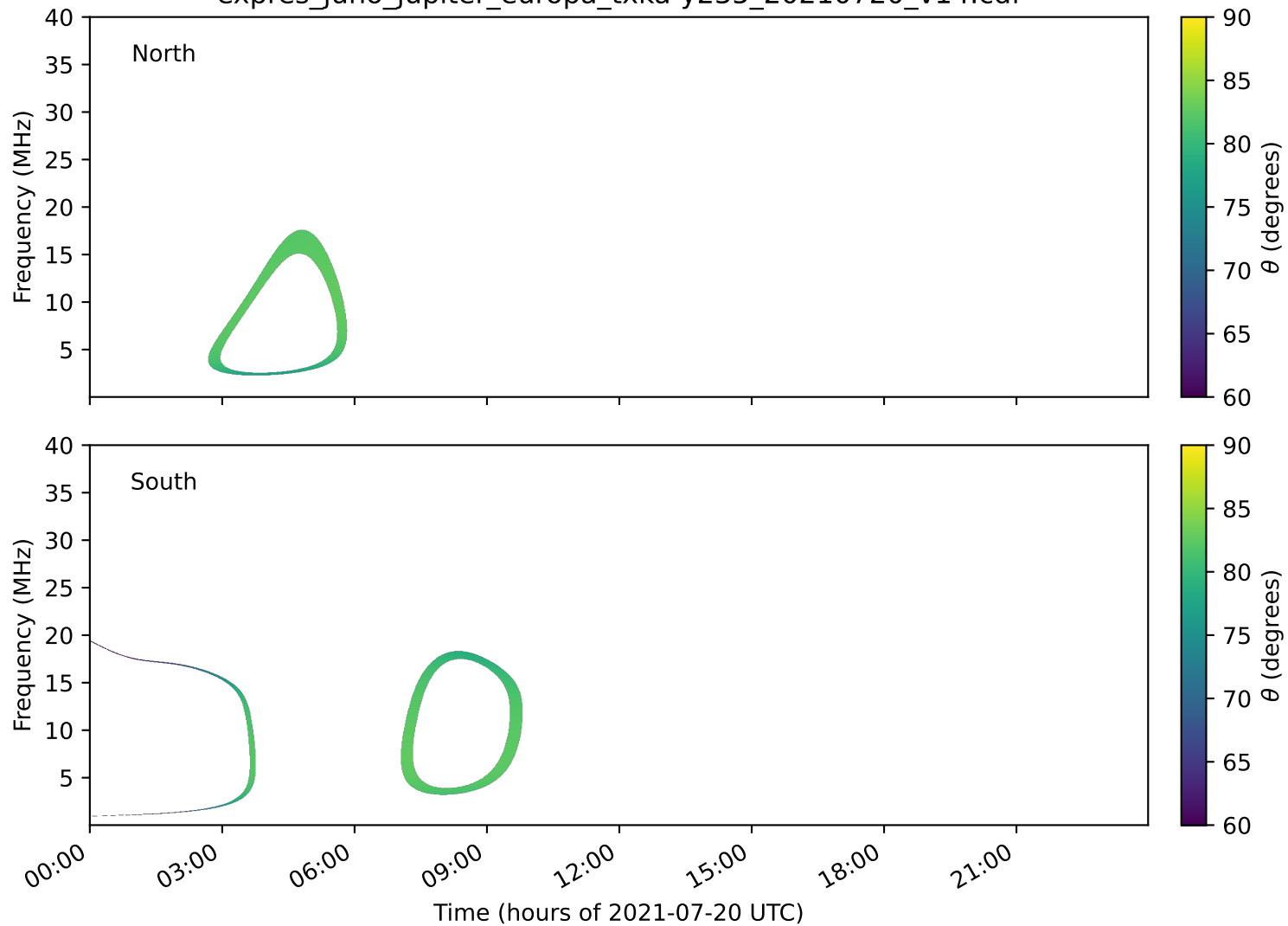
expres_juno_jupiter_europa_txka-y235_20210720_v14.cdf
