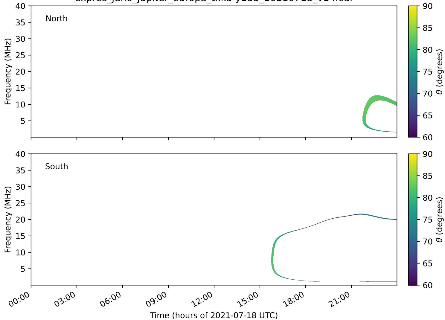
expres_juno_jupiter_europa_txka-y235_20210718_v14.cdf
