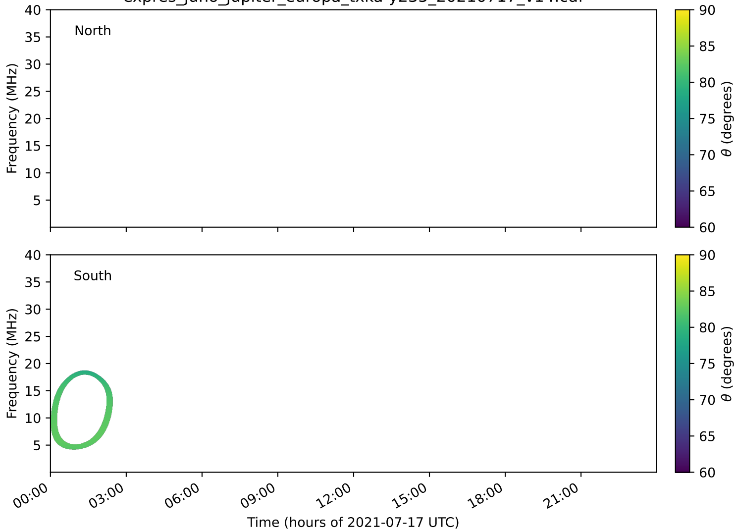
expres_juno_jupiter_europa_txka-y235_20210717_v14.cdf
