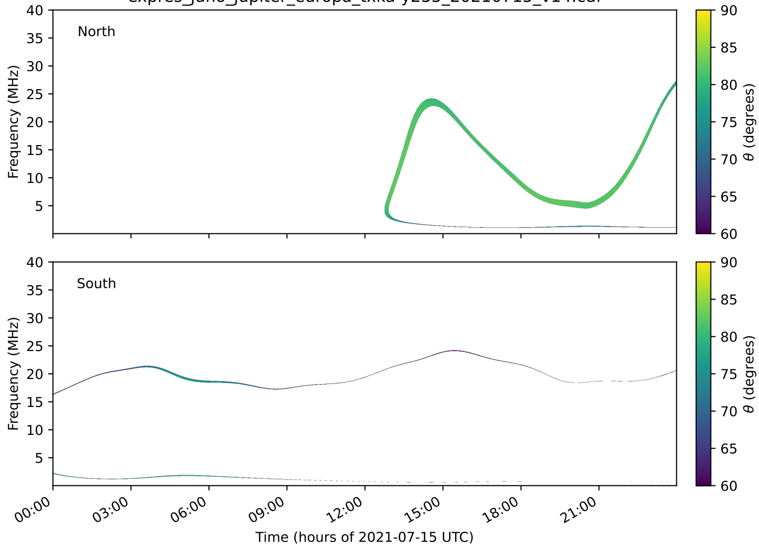
expres_juno_jupiter_europa_txka-y235_20210715_v14.cdf
