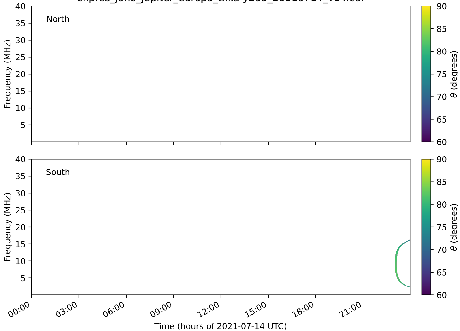
expres_juno_jupiter_europa_txka-y235_20210714_v14.cdf
