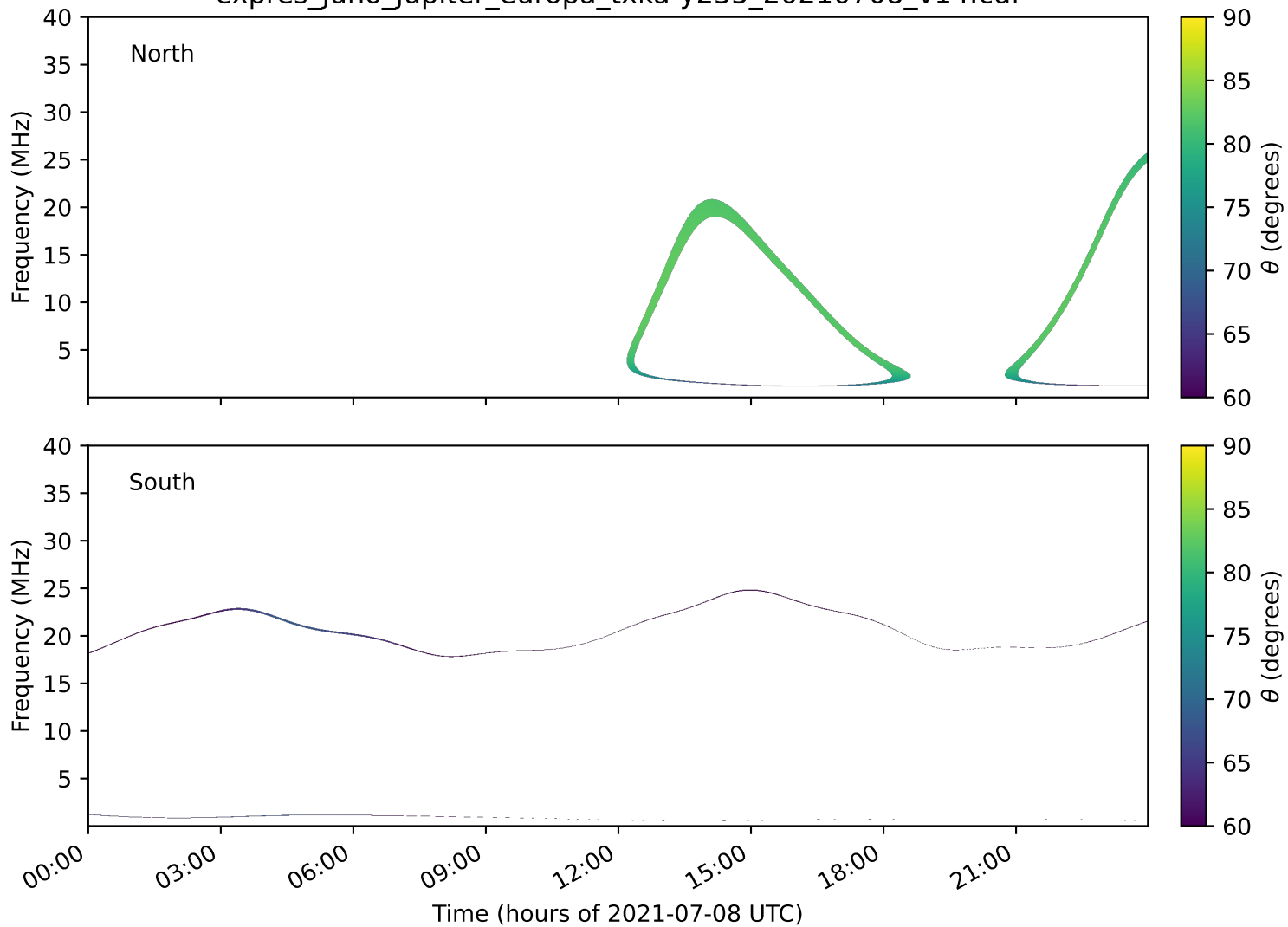
expres_juno_jupiter_europa_txka-y235_20210708_v14.cdf
