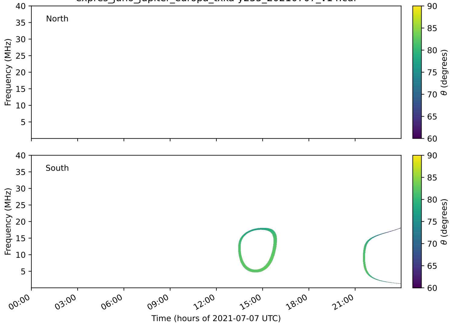
expres_juno_jupiter_europa_txka-y235_20210707_v14.cdf
