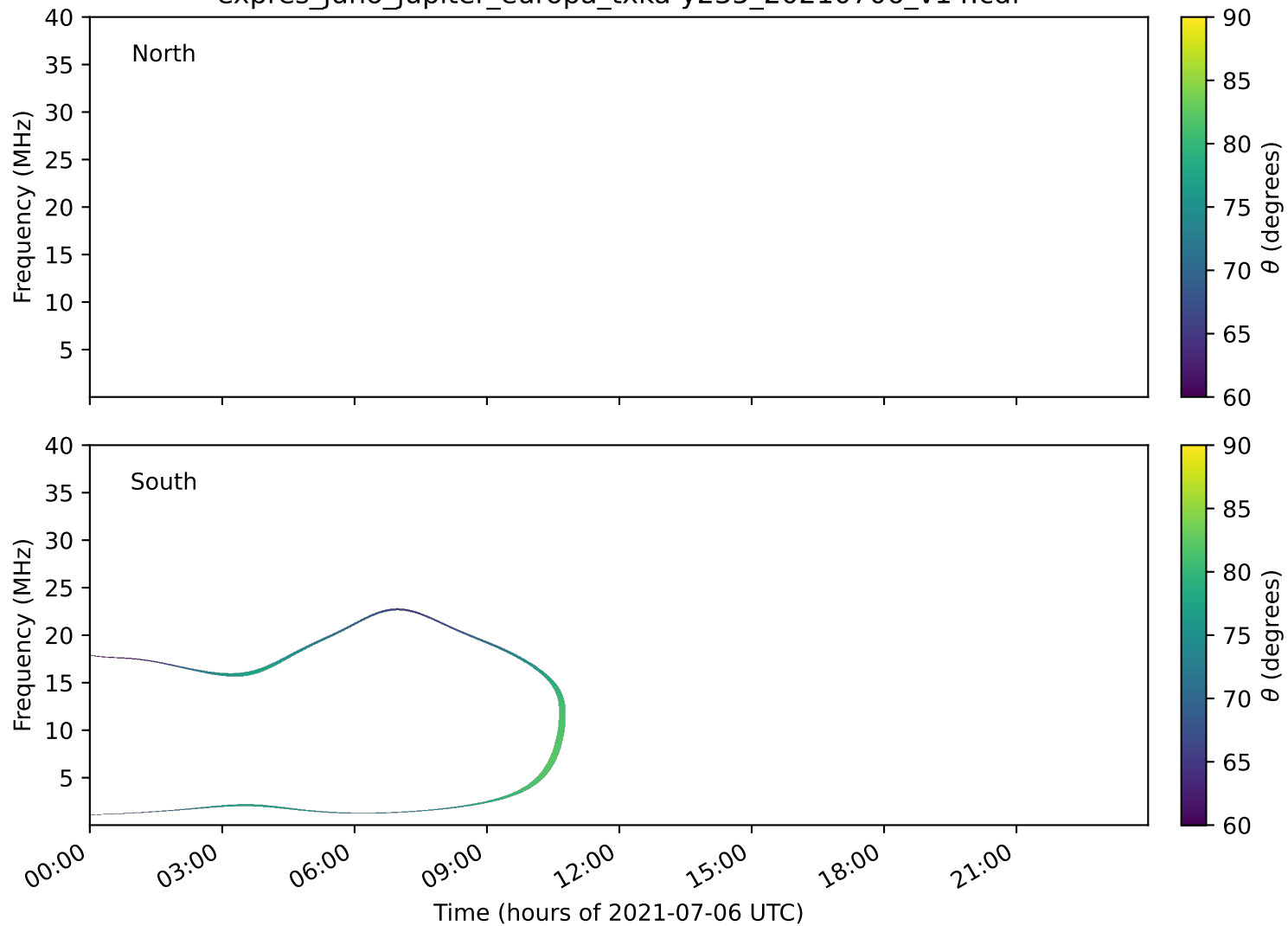
expres_juno_jupiter_europa_txka-y235_20210706_v14.cdf
