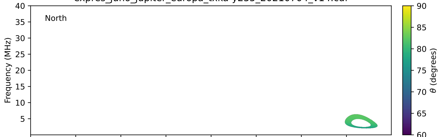
expres_juno_jupiter_europa_txka-y235_20210704_v14.cdf
