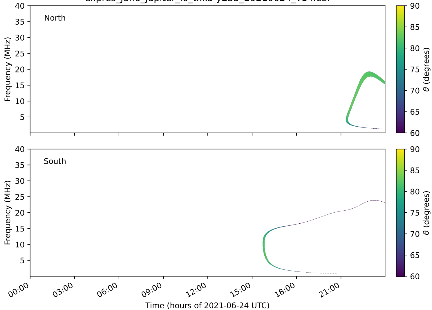
expres_juno_jupiter_io_txka-y235_20210624_v14.cdf
