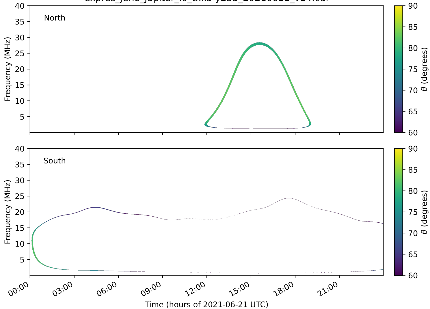
expres_juno_jupiter_io_txka-y235_20210621_v14.cdf
