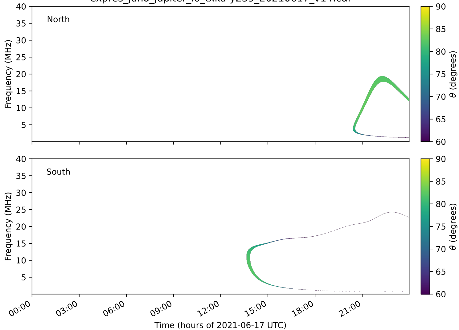
expres_juno_jupiter_io_txka-y235_20210617_v14.cdf
