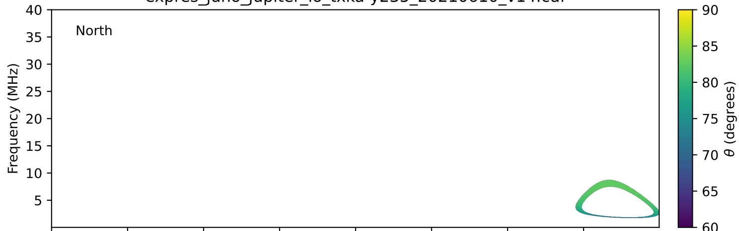
expres_juno_jupiter_io_txka-y235_20210610_v14.cdf
