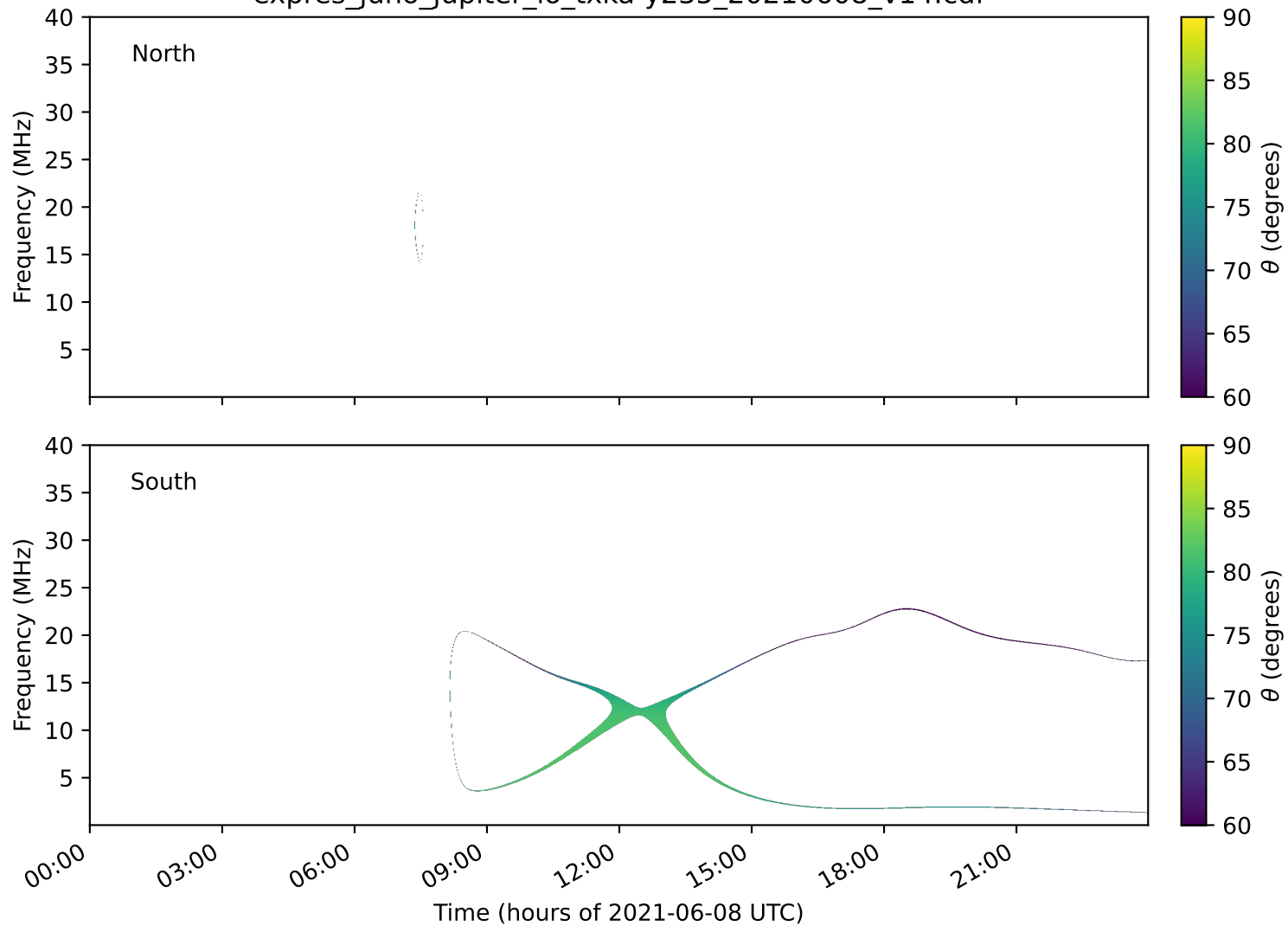
expres_juno_jupiter_io_txka-y235_20210608_v14.cdf
