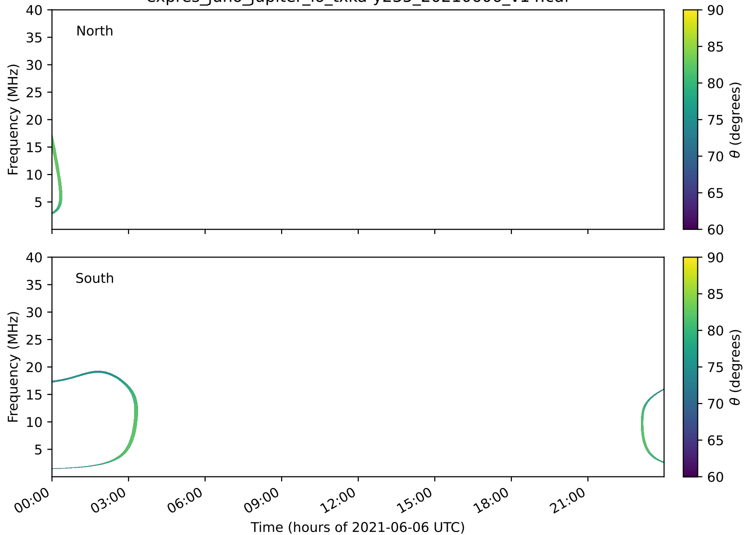
expres_juno_jupiter_io_txka-y235_20210606_v14.cdf
